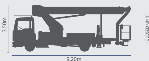
Side profile
